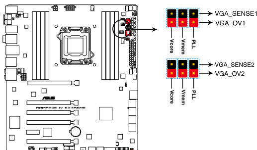
RAMPAGE IV EXTREME VGA Hotwire connectors
