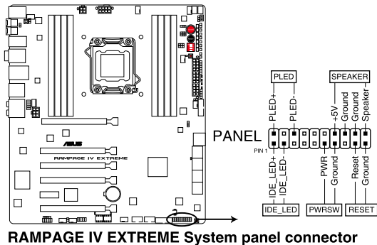
RAMPAGE IV EXTREME System panel connector
